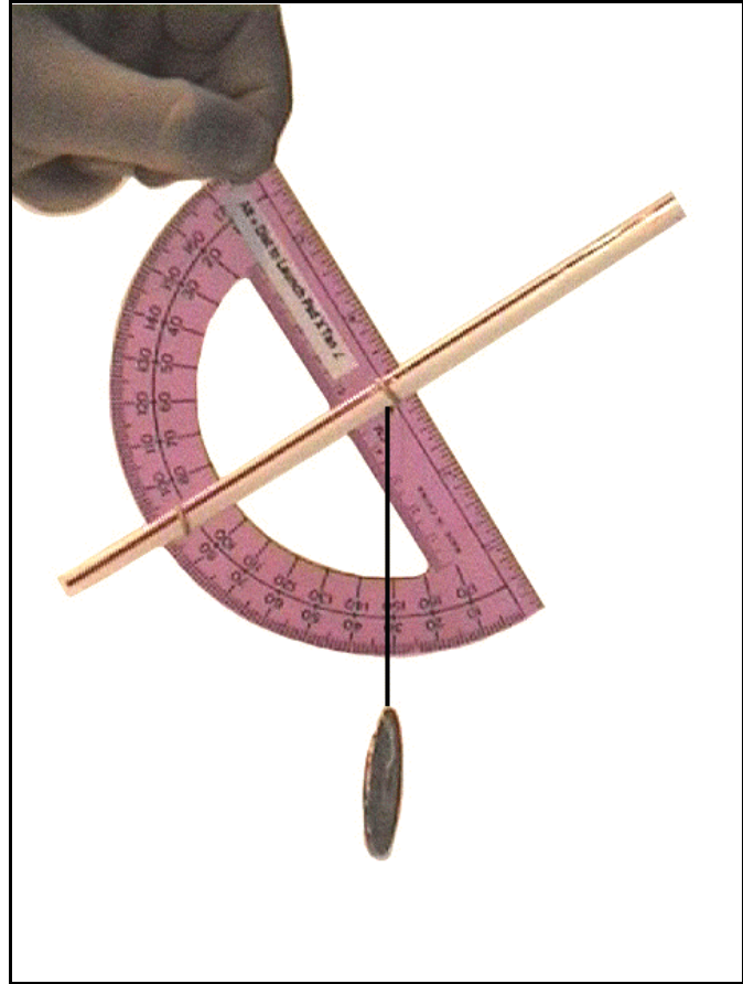
Figure 13: Simple Clinometer
