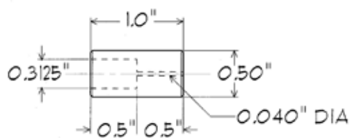
(C) ALUMINUM FERRULE
